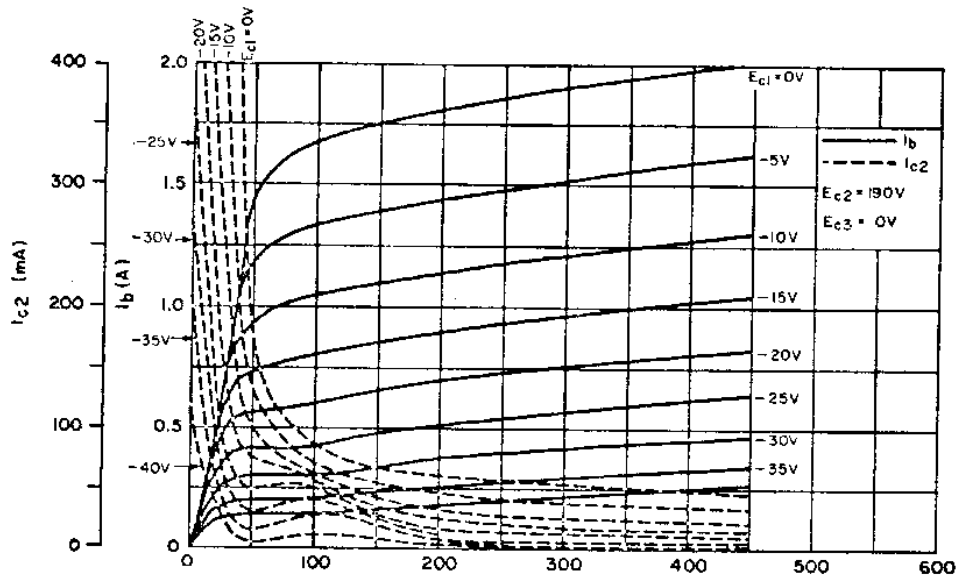
Plate Characteristics
