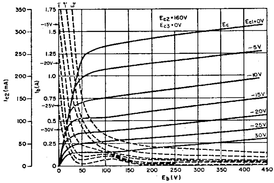
Plate Characteristics
