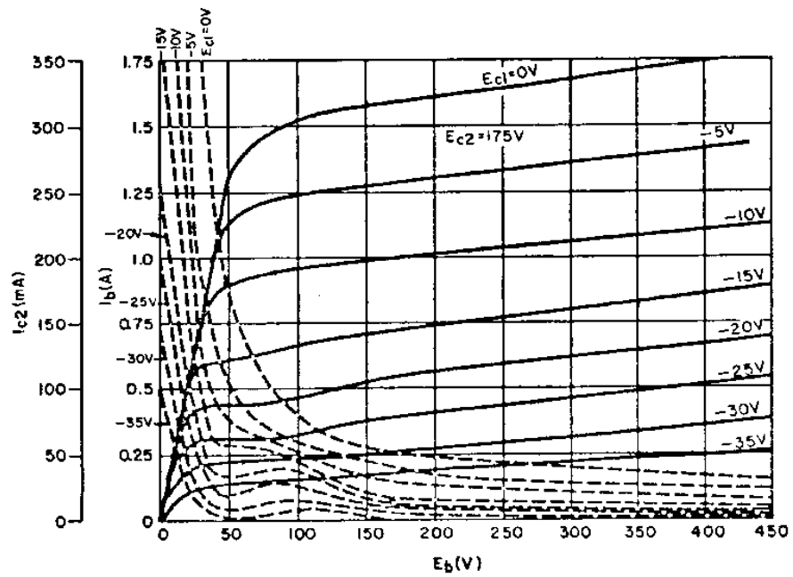
Plate Characteristics
