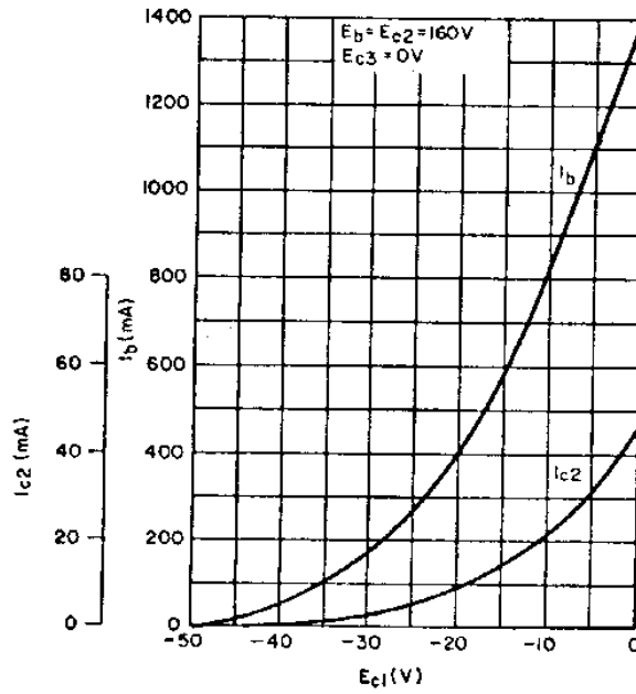
Transfer Characteristics
